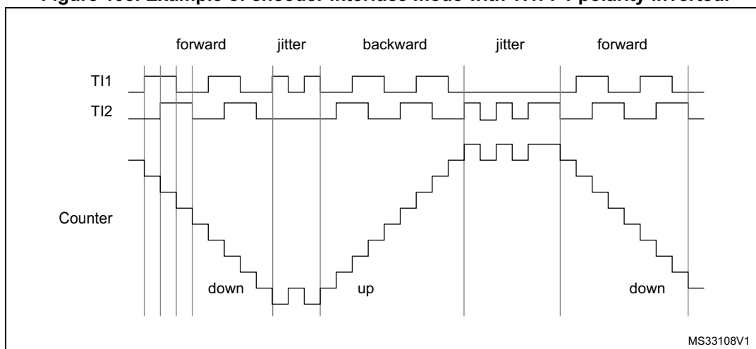
Figure 105. Example of encoder interface mode with TI1FP1 polarity inverted.
