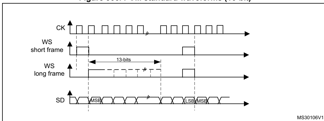
Figure 306. PCM standard waveforms (16-bit)
