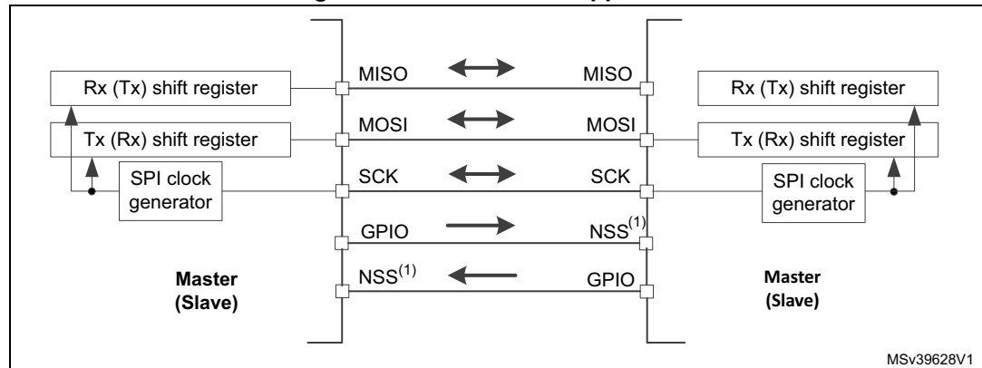
Figure 278. Multi-master application
