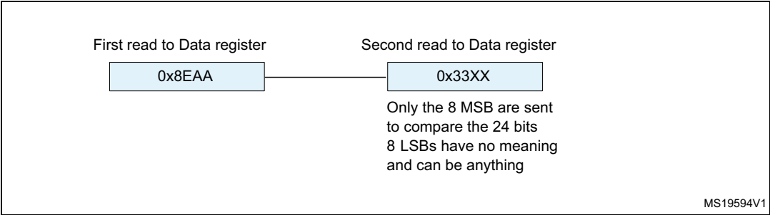
Figure 294. Receiving 0x8EAA33
