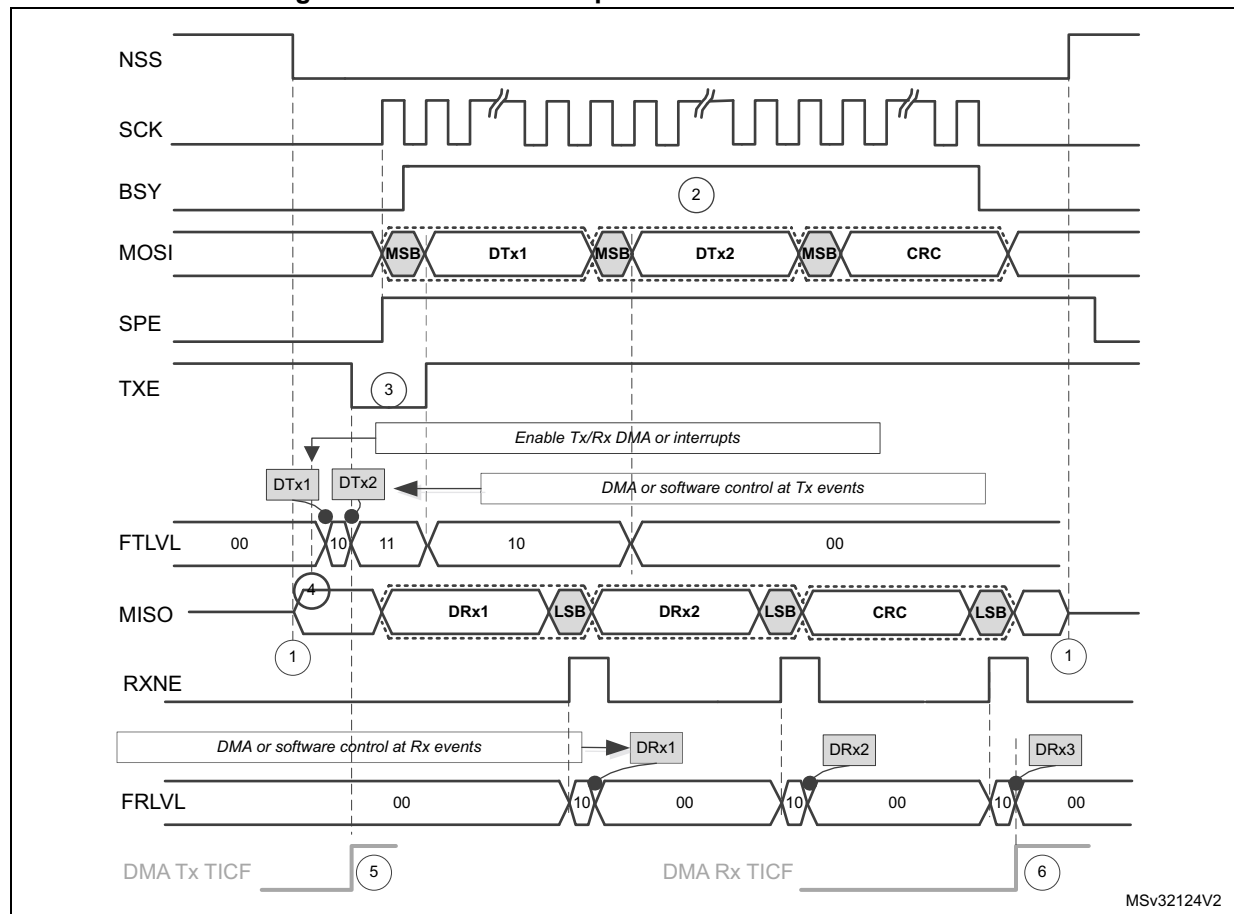
Figure 285. Master full-duplex communication with CRC
