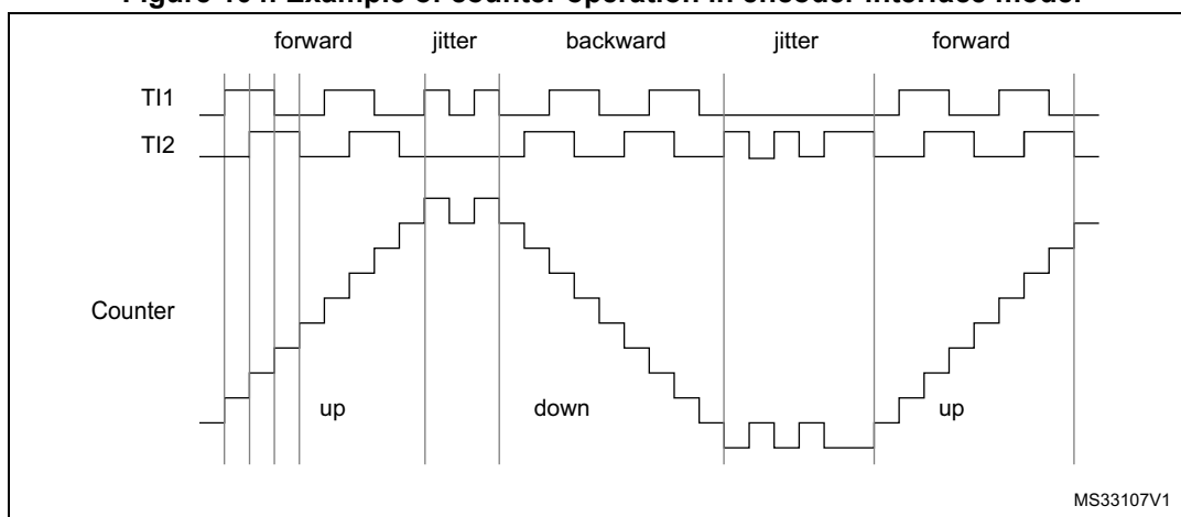
Figure 104. Example of counter operation in encoder interface mode.
