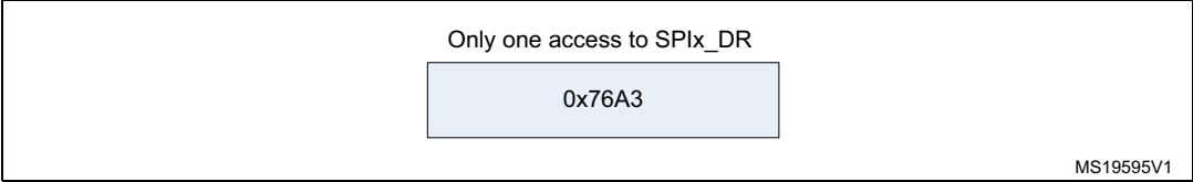
Figure 296. Example of 16-bit data frame extended to 32-bit channel frame
