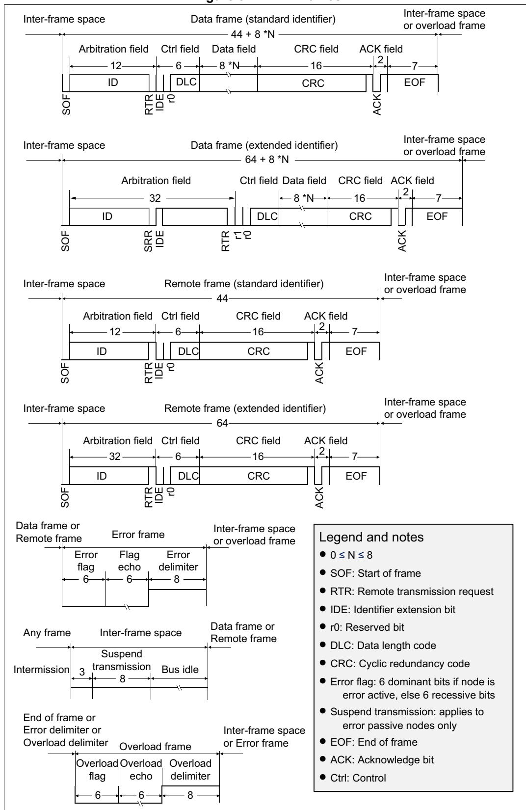
Figure 324. CAN frames
