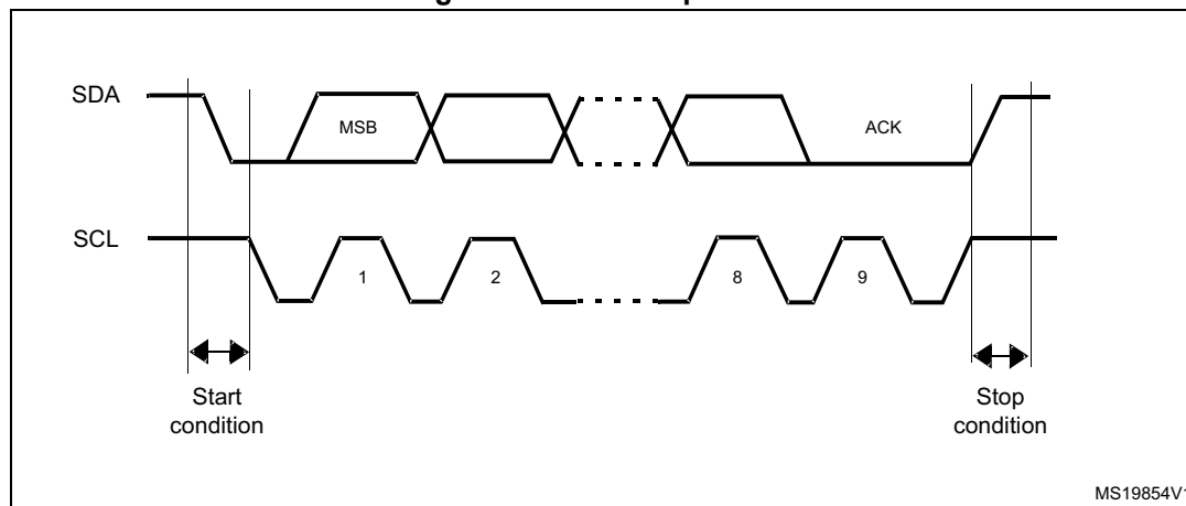
Figure 219. I 2 C bus protocol
