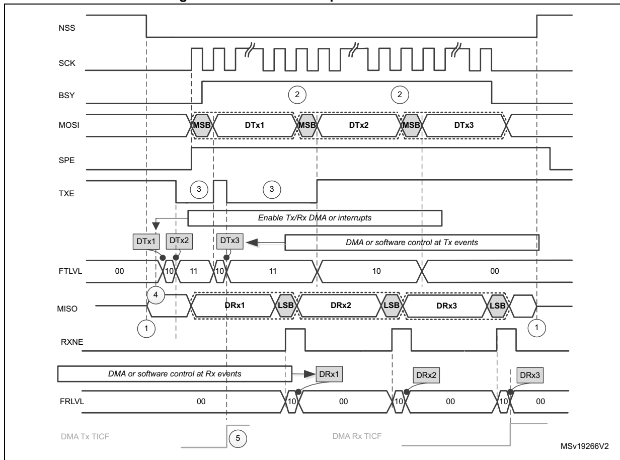
Figure 283. Master full-duplex communication
