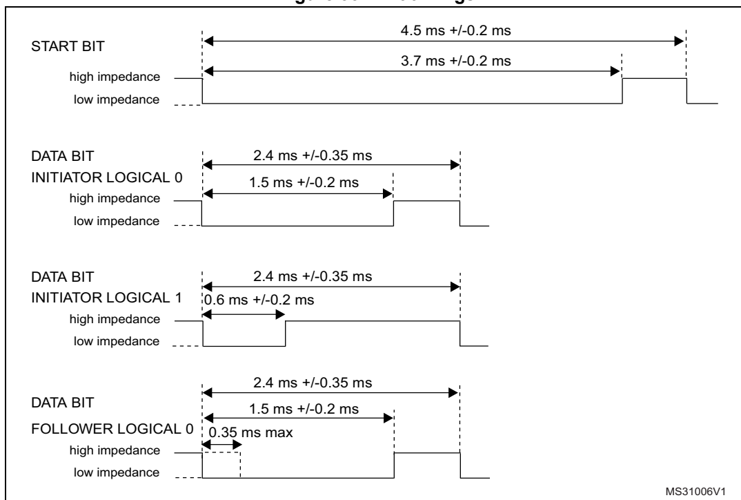
Figure 332. Bit timings
