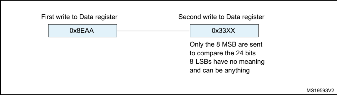
Figure 293. Transmitting 0x8EAA33
